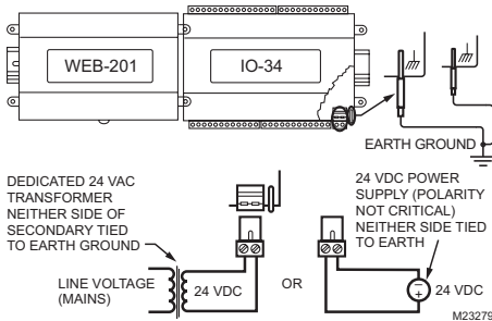
Fig. 4. WEB-IO-34 earth ground connection.
