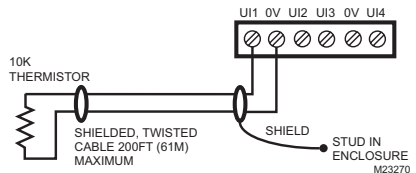
Fig. 5. Thermistor wiring.
